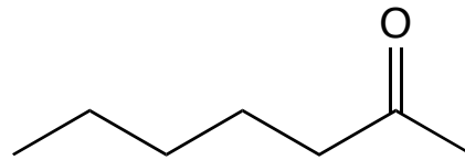
2-eptanone
