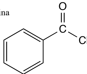
benzoil cloruro
