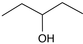
pentan-3-olo
